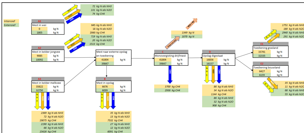
Figuur B3.2 Scenario 2: Regulier + monovergisting.
