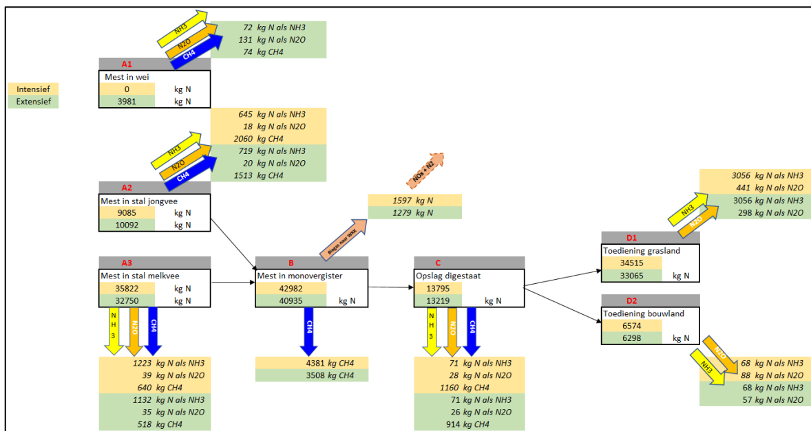
Figuur B3.7 Scenario 6: Dagontmesting + monovergisting.
