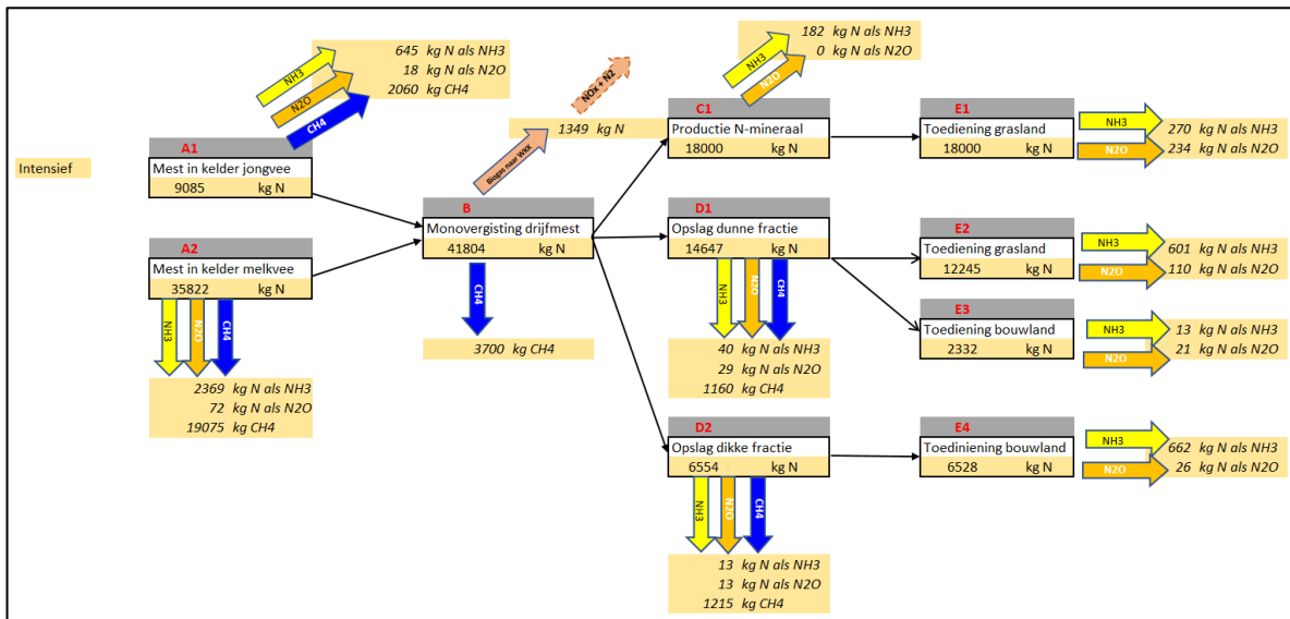
Figuur B3.3 Scenario 3: Regulier + monovergisten + strippen.
