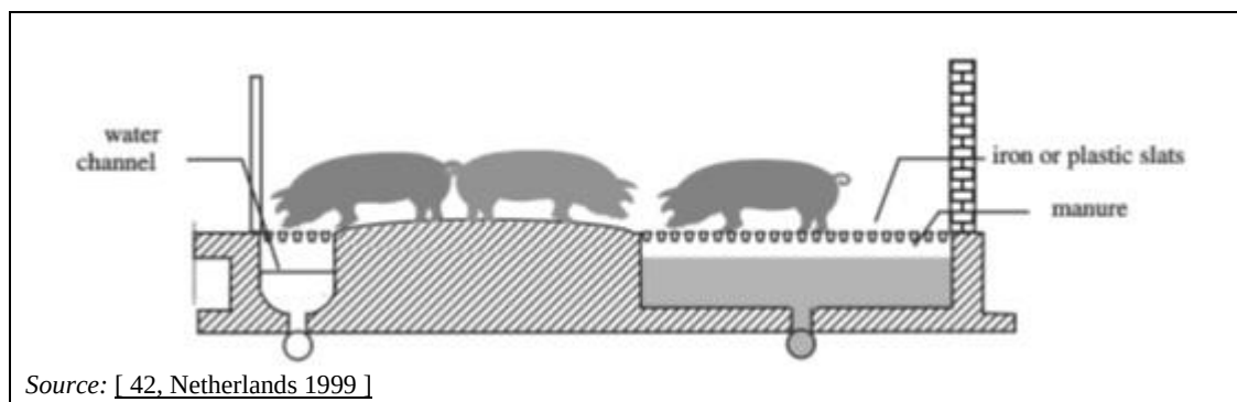
Figure 4.53: Partly slatted floor with a shallow manure pit and a water channel for spoiled drinking water in combination with a convex floor
