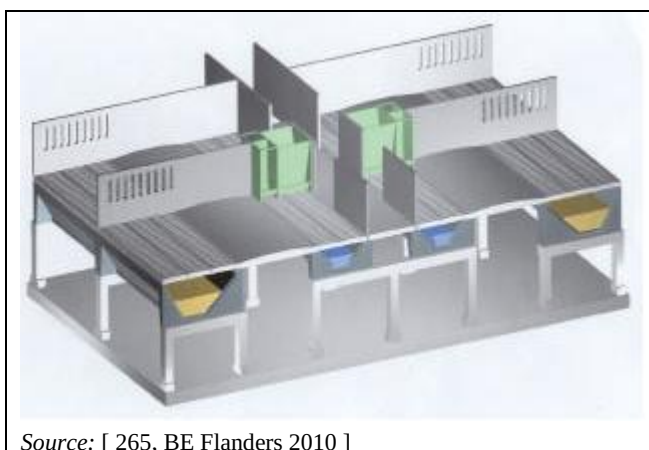
Figure 2.20: Pen design for fattening pigs with partly slatted (convex) floor and solid area in the centre
