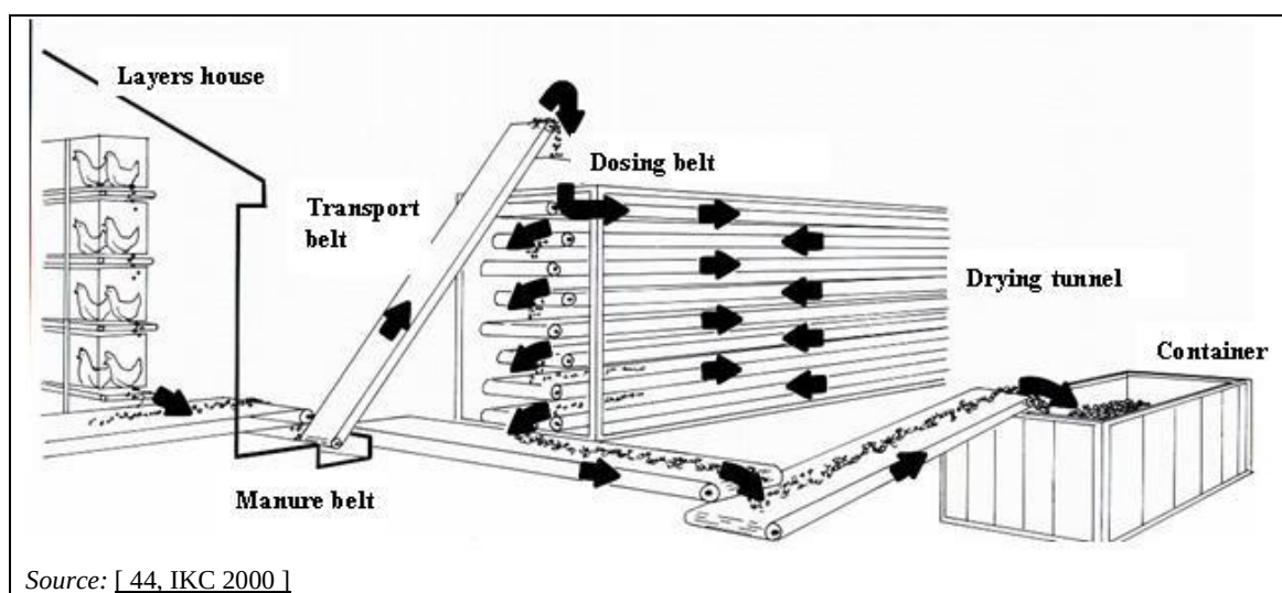
Figure 4.89: Principle of external drying tunnel with perforated manure belts
