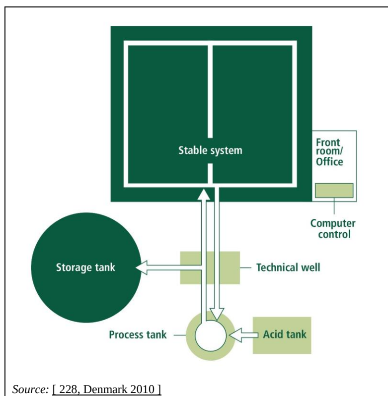
Figure 4.90: Schematic representation of a slurry acidification system
