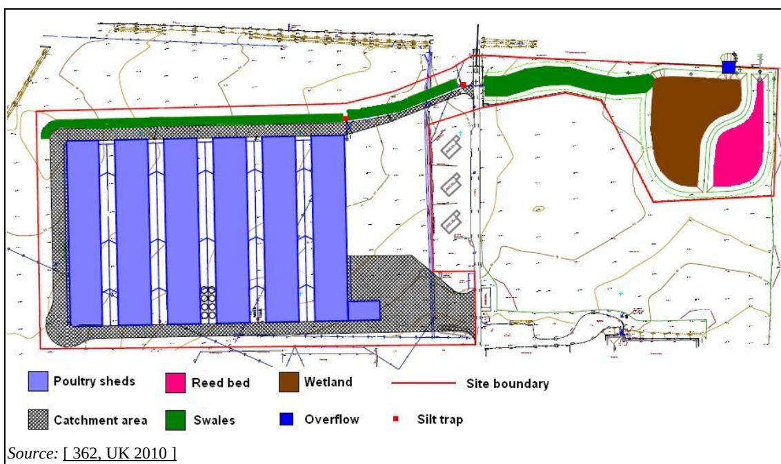
Figure 4.103: Location of a system of swales and wetland for a poultry farm
