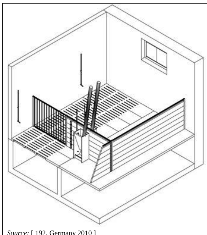
Figure 2.19: Design of a partly slatted floor system for fattening pigs
