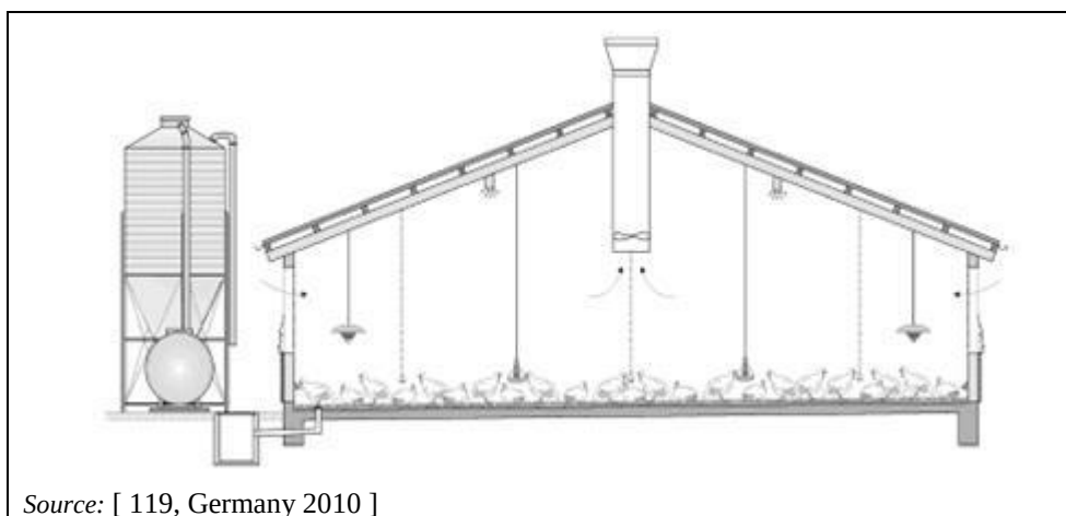
Figure 4.26: Scheme of a naturally ventilated house for turkey fattening
